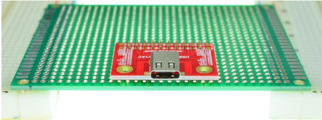
Figure 3: Solid Mounting on prototype PCB
